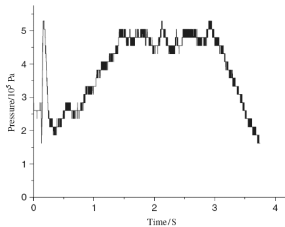
Figure 3.3: The whole pressure curve measured by the pressure sensor installed on the top of the vessel (60% liquid height; 130 °C; 6.67% orifice area)
