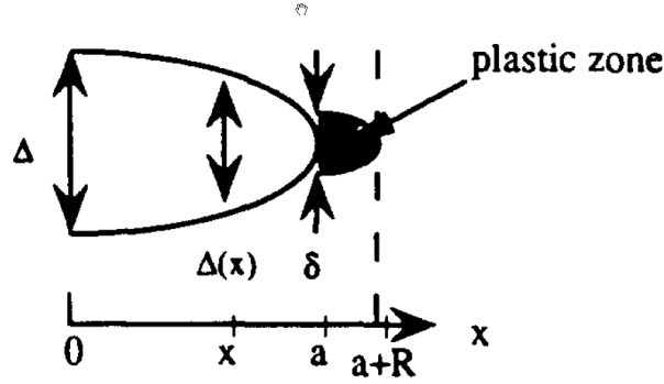
Figure 3.1: Crack displacement concept
