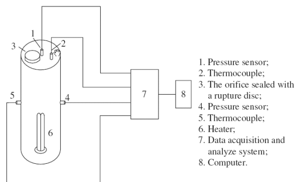
Figure 3.2: Experimental setup
