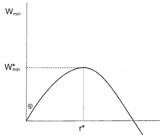
Figure 1.1: The variation of W_{min} , the Gibbs formation energy of a cluster of molecules form a bubble nucleus, as function of the radius of such clusters and the nucleation barrier W_{min}^*
