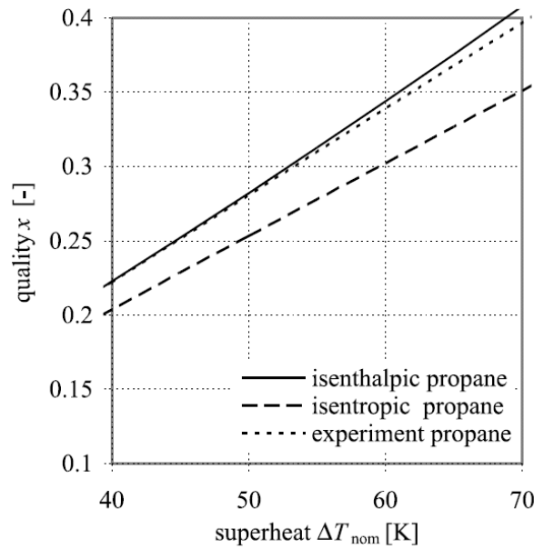
Figure 3.7: Isenthalpic, isentropic and experimental quality x for propane
