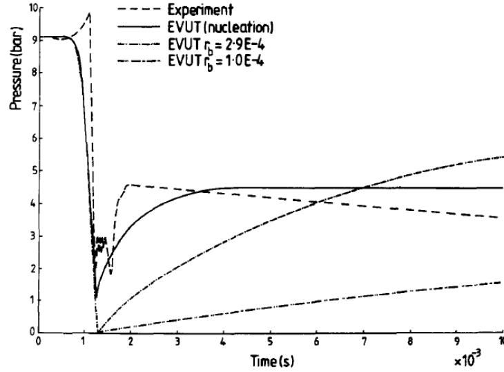
Figure 3.9: Initial depressurization
