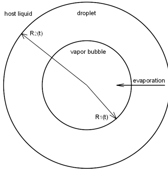
Figure 2.1: Schematic illustration of explosive boiling of a liquid droplet
