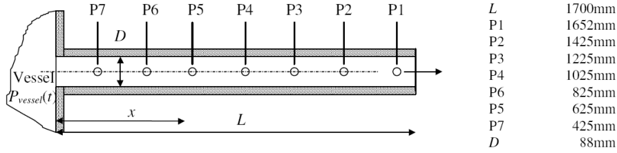
Figure 3.6: Schematic description of the experimental channel, [2]
