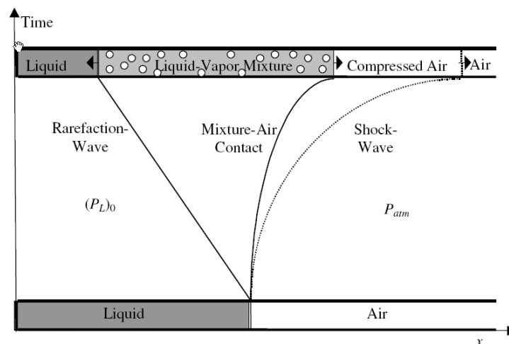
Figure 3.10: Typical wave action in the x - t plane following BLEVE
