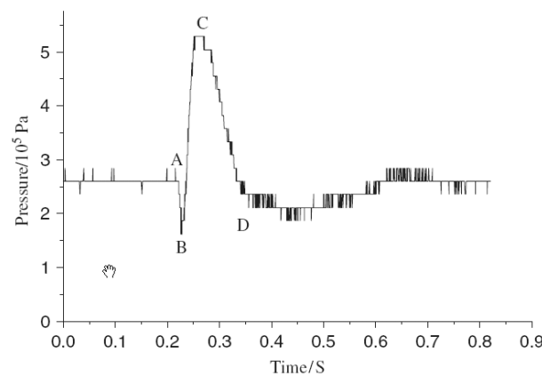
Figure 3.4: The enlarge diagram of the first pressure peak in Fig.(3.3).
