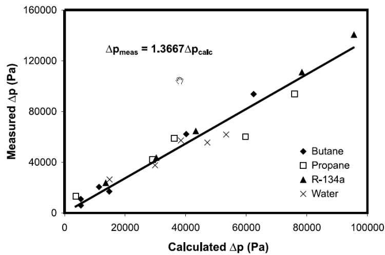
Figure 3.8: Comparison of the predicted press drop with measured values
