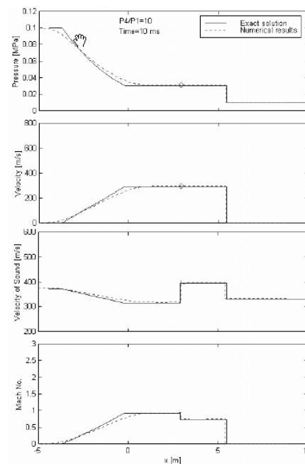
Figure 3.11: Profile of the flow properties for test case p_L/p_R = 10 at time t = 10 \text{ ms}
