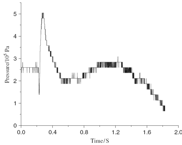
Figure 3.5: The whole pressure curve measured by the pressure sensor installed in the wall of the vessel at middle height (60% liquid height; 130 °C; 6.67% orifice area)
