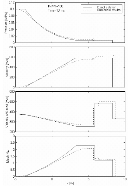
Figure 3.12: Profile of the flow properties for test case p_L/p_R = 100 at time t = 10\text{ ms}
