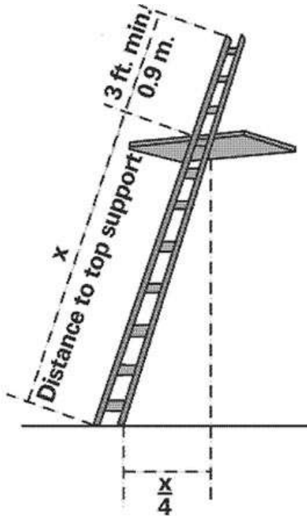
Figure D-1 -- Portable Ladder Set-up
